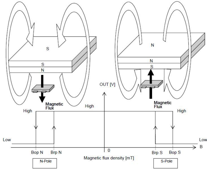
Fig 4, Magnetic Operation Characteristic of AS1805
